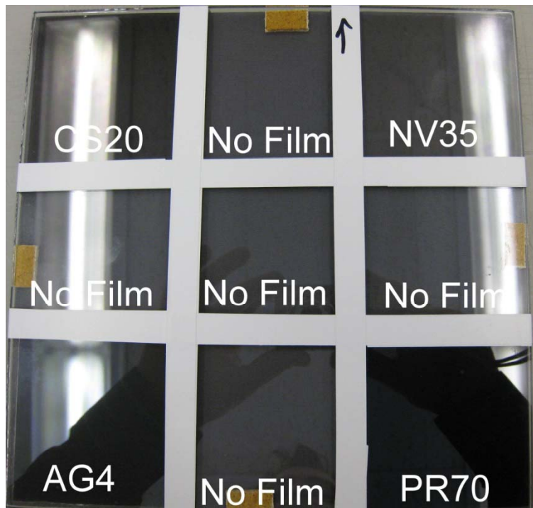
Black Surface Before vs. After Exposure to UV
